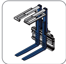
带货物稳定器的单双托盘叉 适合搬运单层堆垛货物 Single-Double with Load Stabilizer for single high stacks
