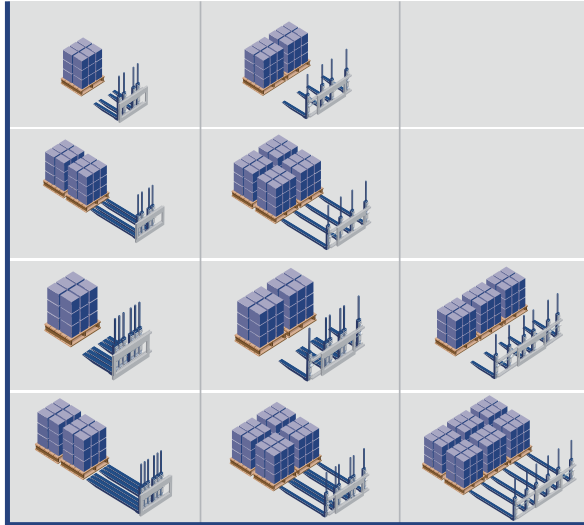
单双三托盘叉 FTS型-可同时搬运1、2或3个托盘 Single-Double-Triple Pallet Handler Model FTS • 1-2-3 Pallets
