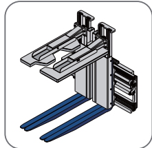
带货物压紧器的单双托盘叉 适合搬运双层堆垛货物 Single-Double with Load Hold-Down for double high stacks
